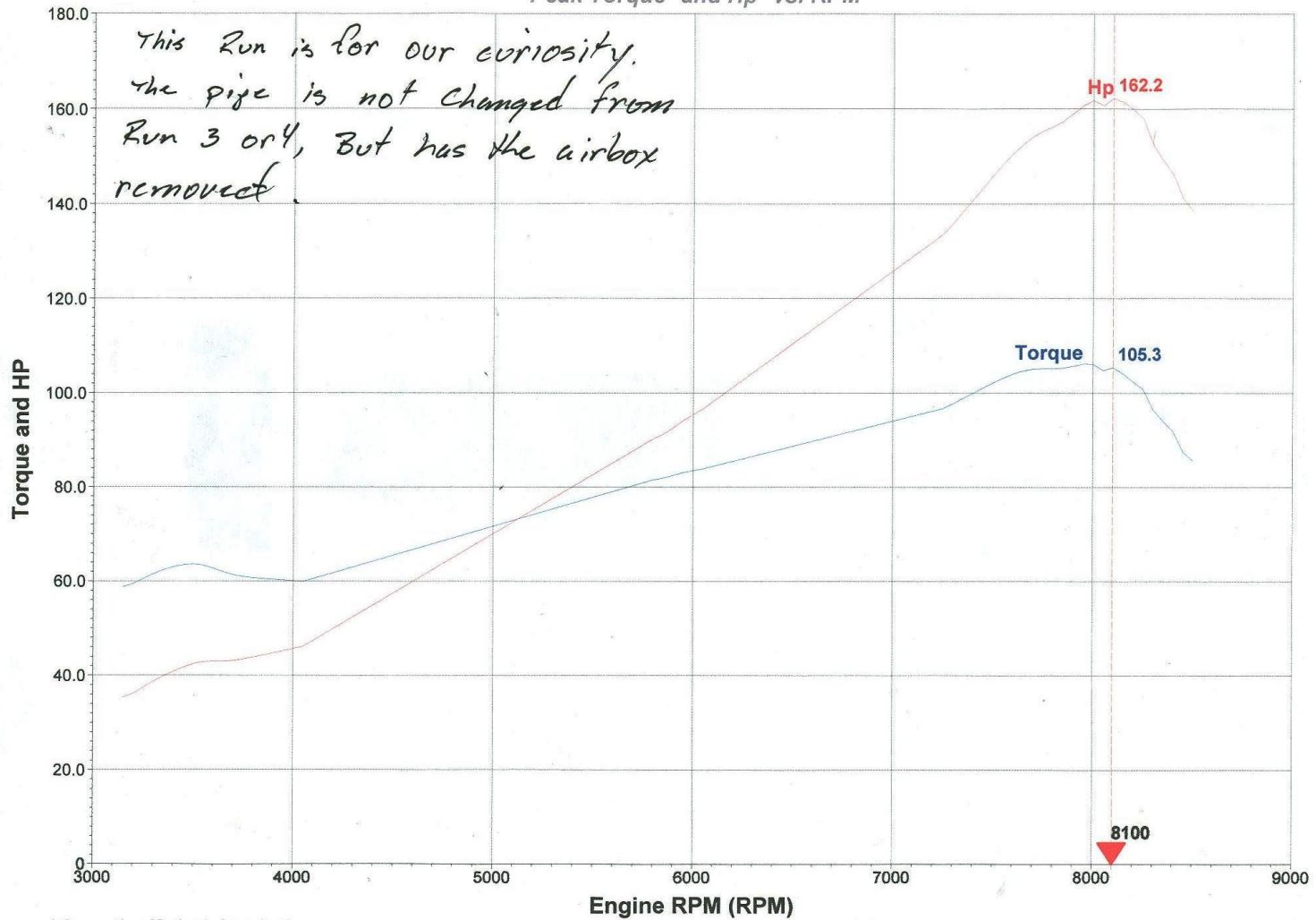
Peak Torque* and Hp* vs. RPM
