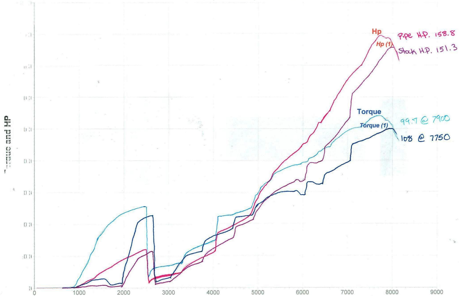
Peak Torque* and Hp* vs. RPM
