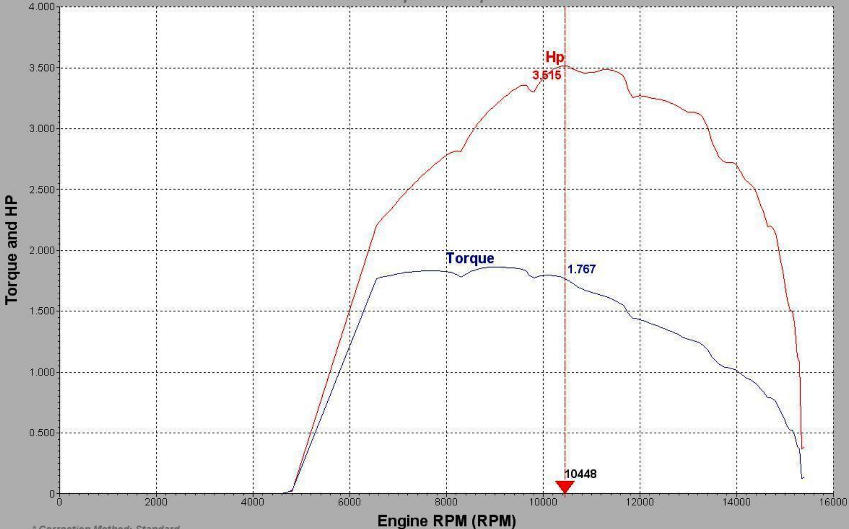
Peak Torque* and Hp* vs. RPM
